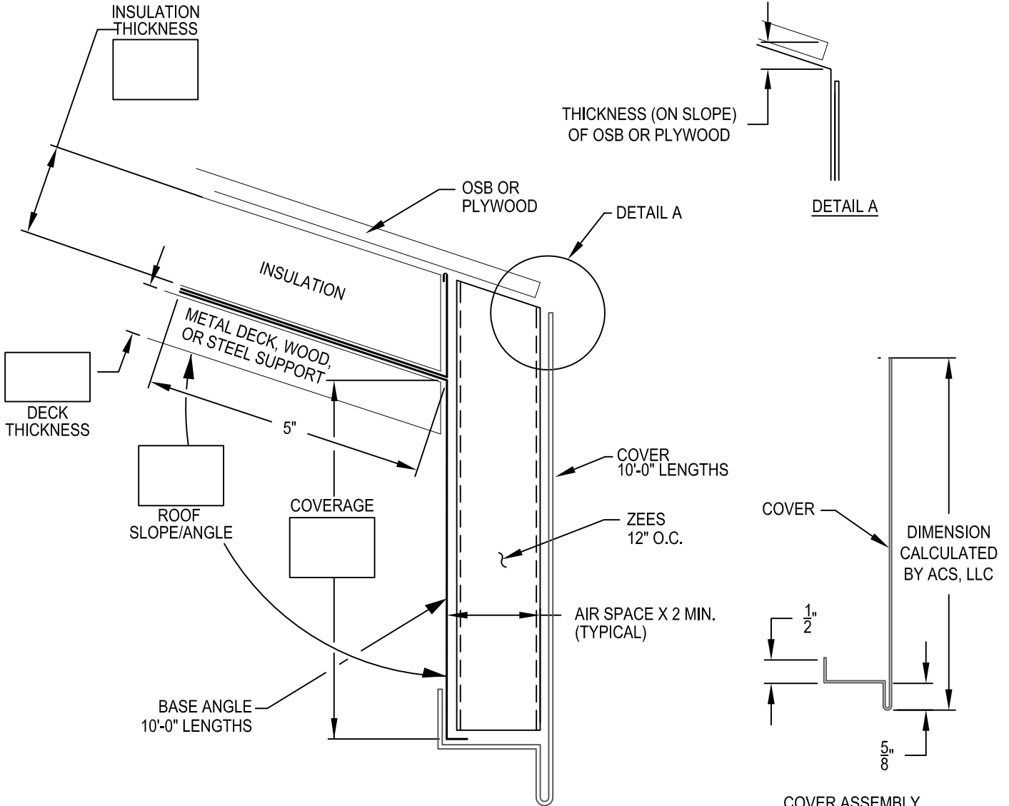
COVER ASSEMBLY NOTE: COVER INCLUDES 3" SPLICE PLATES
